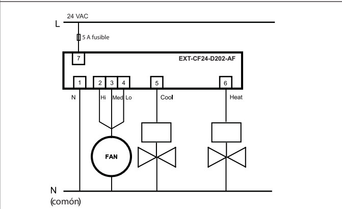
Control On/Off - 2 Cables
