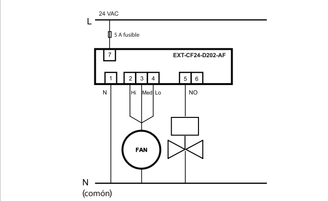
On-Off - 2 Cables
