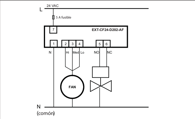
On-Off - 3 Cables
