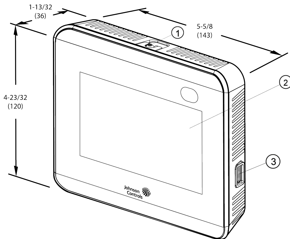
Figure 2: Thermostat shown without occupancy sensor, dimensions, in. (mm)
