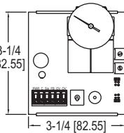
Shown with snap-track mounting
