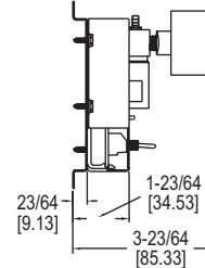
Shown with metal bracket mounting
