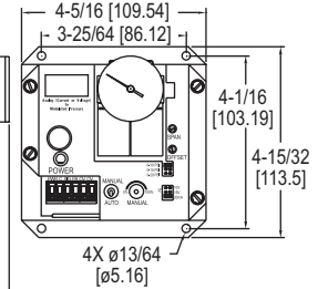
Shown with metal bracket mounting
