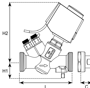
FlowCon EVS in FlowCon ABV1 valve DN15/20/25 (1/2", 3/4", 1") with EV.0.2/1.3/1.4 actuator
